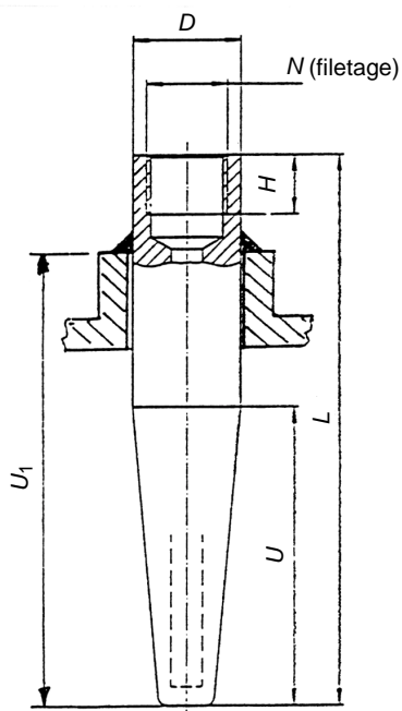
Figure 7 – Type D – Configuration extérieure
