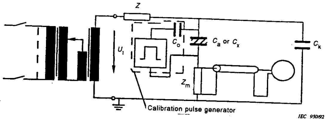
Figure C.4 – Calibration for unearthed test specimen
