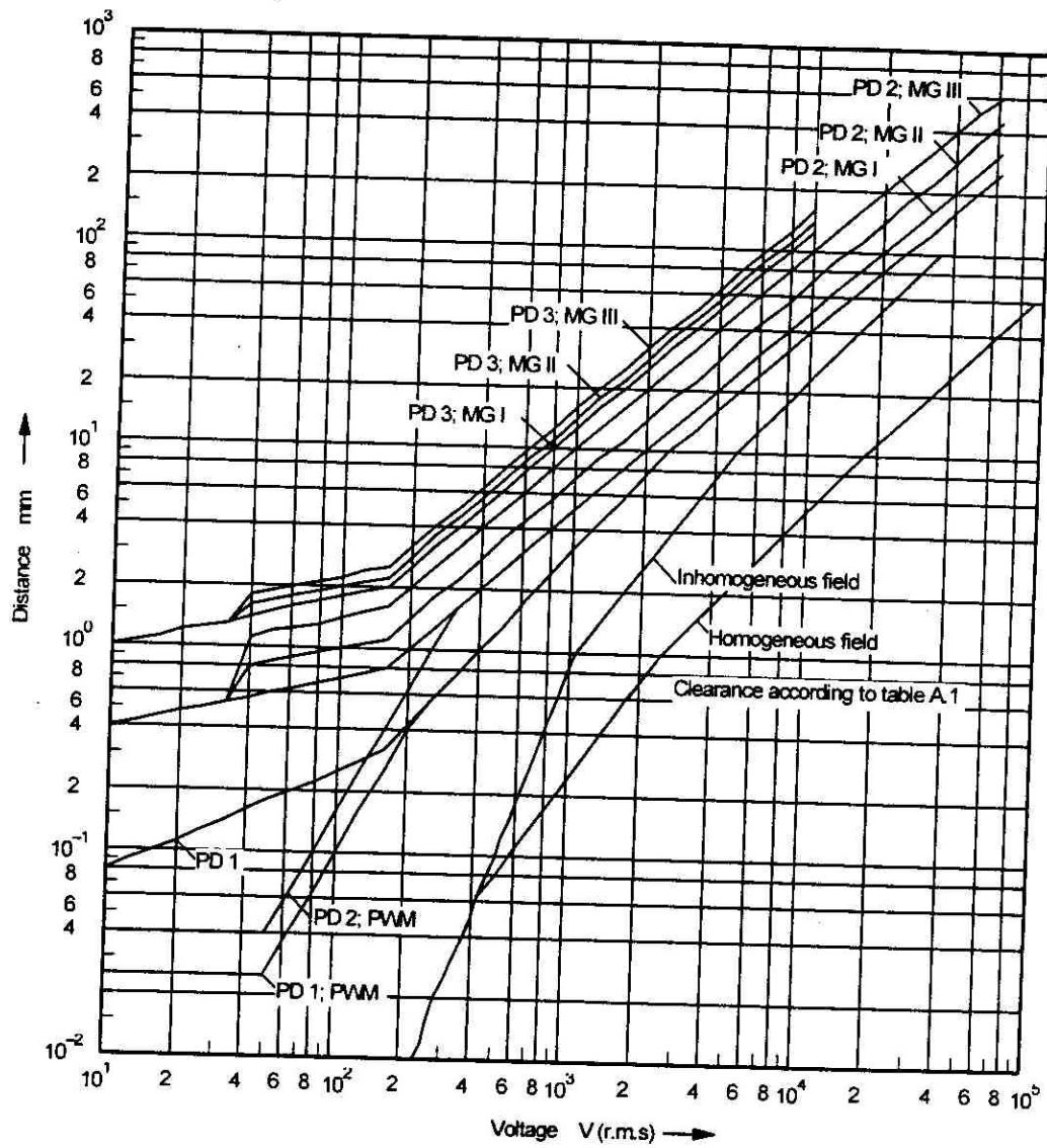
Figure E.1 - Comparison of creepage distances specified in table 4 and clearances in table A.1
