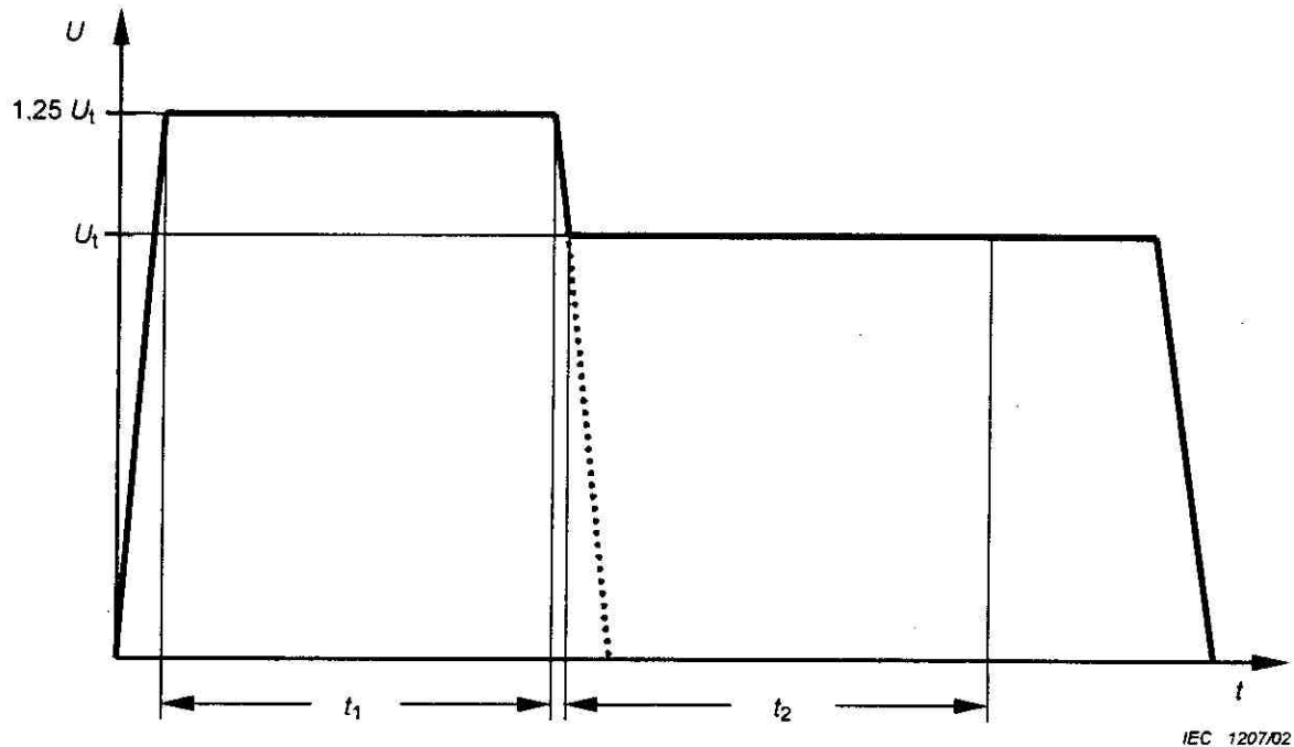
Figure 2 – Test voltages
