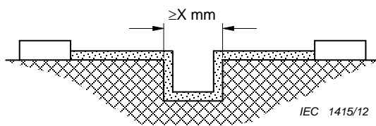
Figure 24 – CREEPAGE DISTANCE and AIR CLEARANCE – Example 3
