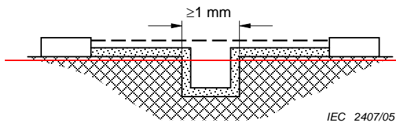
Figure 23 – CREEPAGE DISTANCE and AIR CLEARANCE – Example 2
