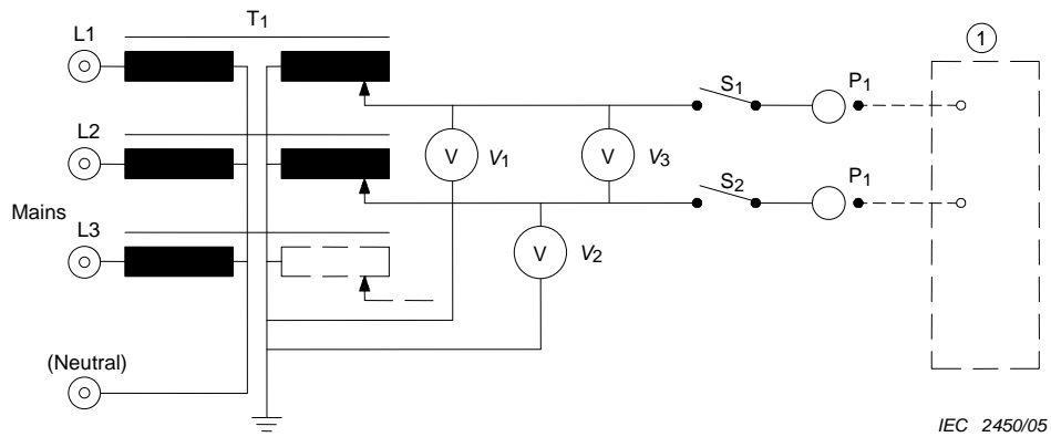
Figure F.3 – Measuring supply circuit for polyphase ME EQUIPMENT specified for connection to a polyphase SUPPLY MAINS (see 8.7.4.2)
