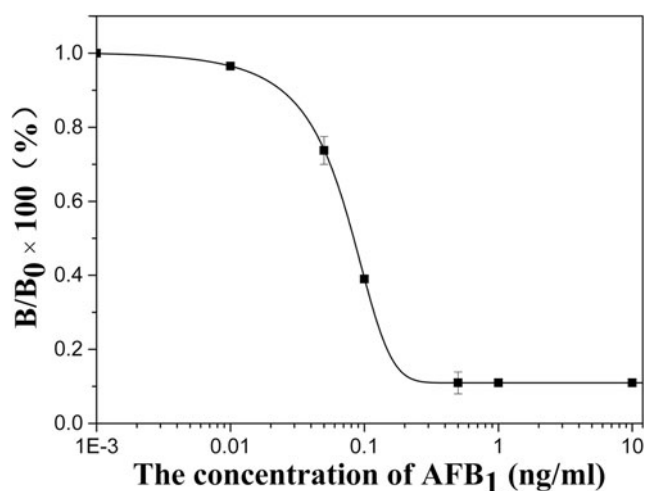
Fig. 3 Inhibition curve for the detection of AFB 1 , where B/B 0 represents the percentage of NSP-DAME-NHS-labeled mAb-AFB 1 specifically bound to the nanoparticles
